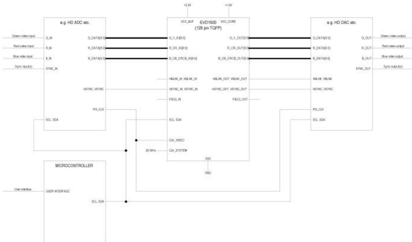
EVD1000 / EVD1500 Simplified Schematic Example: Medical Application
