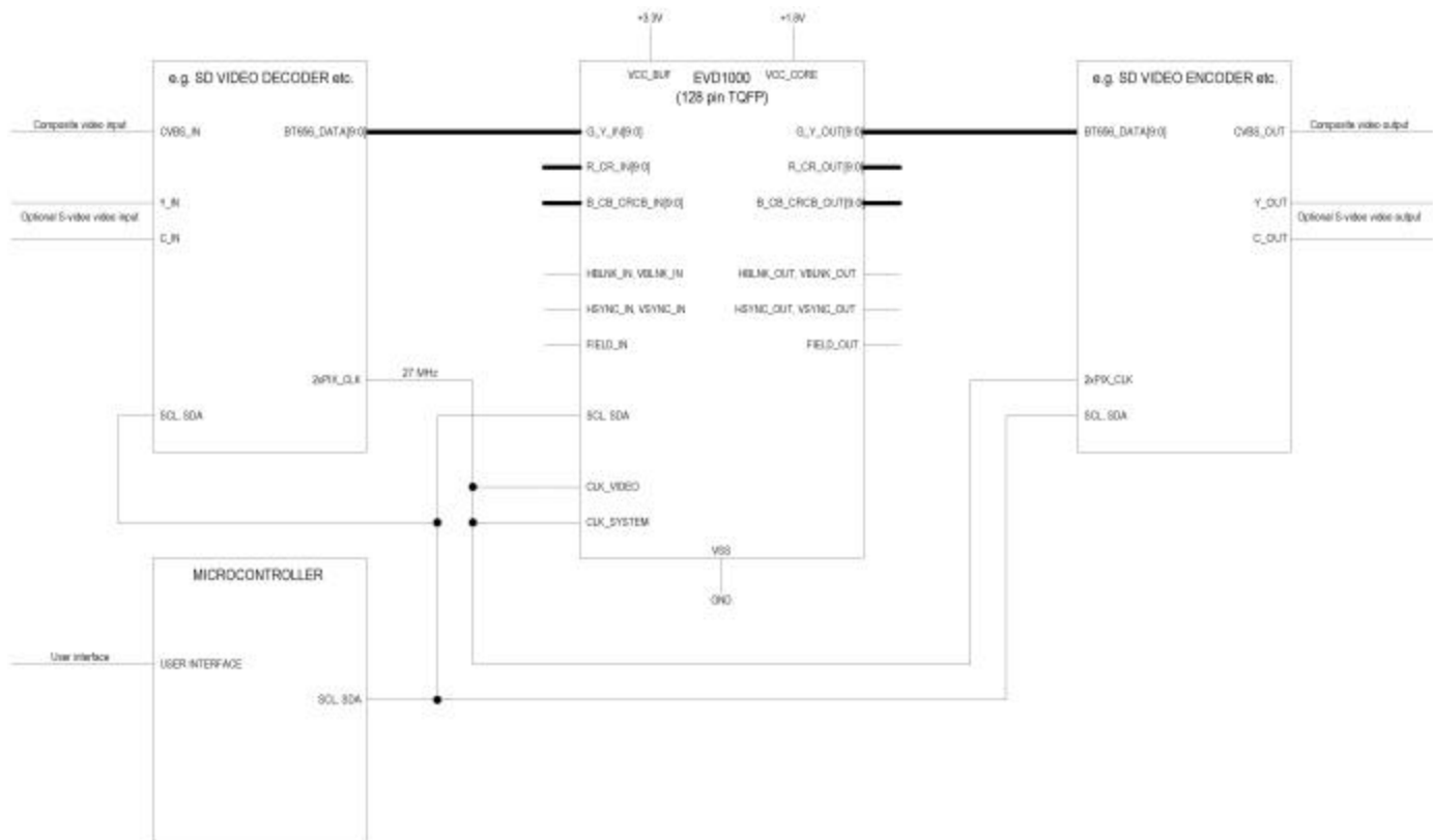
EVD1000 / EVD1500 Simplified Schematic Example: Security Application
